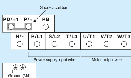
Figure 2. 007SF2 to 022SF2 / 015LF2 to 037LF2 / 004HF2 to 040HF2
