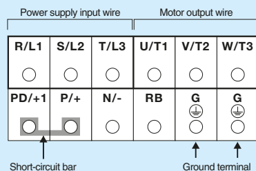
Figure 3. 055LF2, 075LF2, 055HF2, 075HF2, 110LF2, 110HF2, 150HF2, 150LF2
