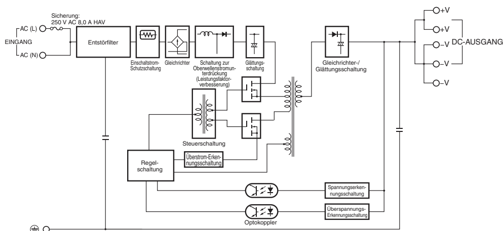
S8VK-C24024 (240 W)
