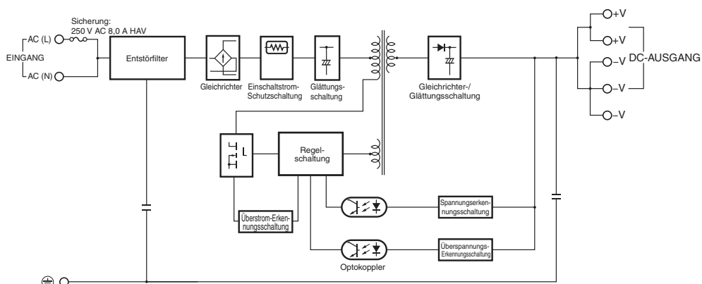
S8VK-C12024 (120 W)
