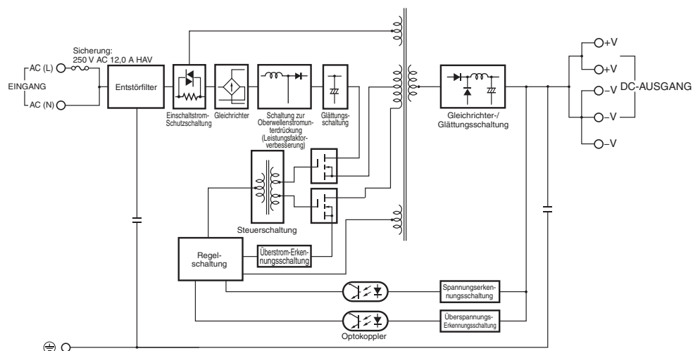
S8VK-C48024 (480 W)
