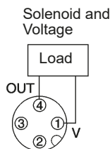
OD0□ Output Connector (NPN)
