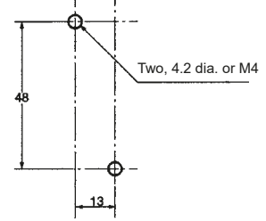
Mounting Holes
