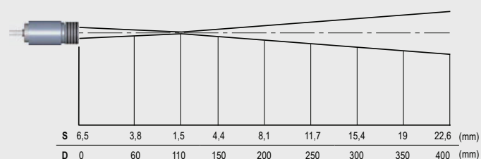
CTi 2MH/2MH1 CF, D:S = 75:1 (Fernfeld = 14:1)
