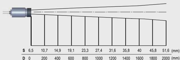
CTi 2ML SF, D:S = 40:1
