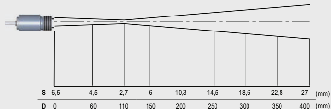
CTi 2ML CF, D:S = 40:1 (Fernfeld = 12:1)
